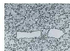
SUS440C (溶製材) 焼入れ: 1030°C × 30min O.Q. Quenching 焼戻し: 500°C × 1h A.C. × 2 Tempering
