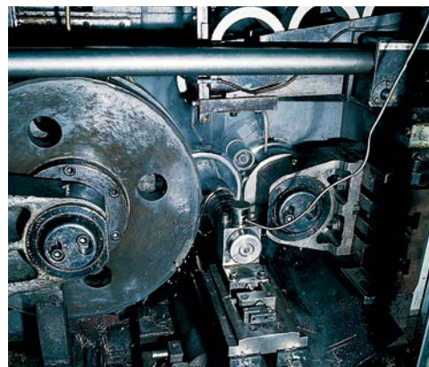
冷間転造機 (CRF) Cold roll forming machine
